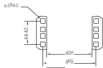
19" mounting
